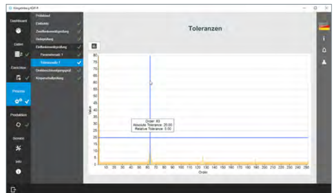
Fig. 3: Tolerance Order Spectra
